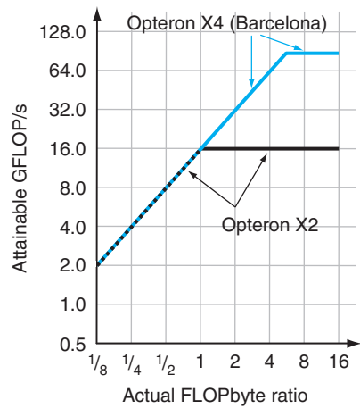
FIGURE 6.19 Roofline models of two generations of Opterons. The Opteron X2 roofline, which is the same as in Figure 6.18, is in black, and the Opteron X4 roofline is in color. The bigger ridge point of Opteron X4 means that kernels that were computationally bound on the Opteron X2 could be memory-performance bound on the Opteron X4.
